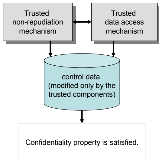
Figure 14: Requirements for Confidentiality Property
