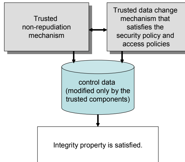
Figure 16: Requirements for Integrity Property
