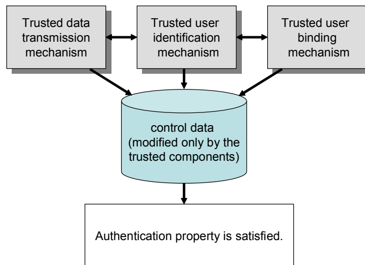
Figure 9: Requirements for Authentication Property
